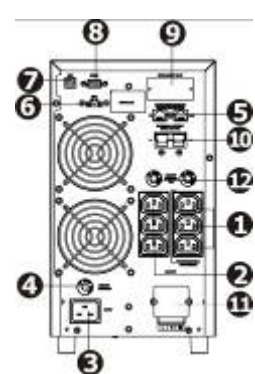
3K(L) TOWER
