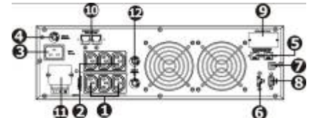
3K(L) RACK
